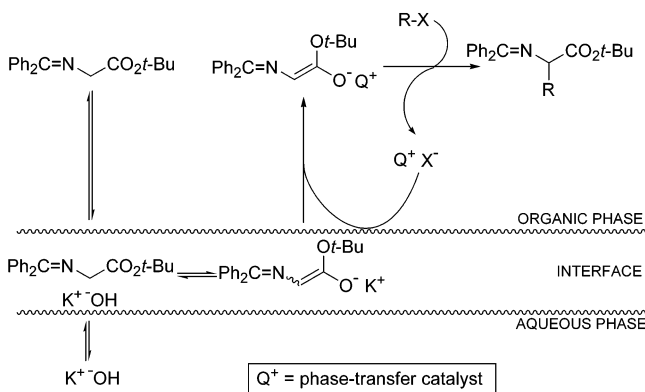
FIGURE 4. Phase-transfer alkylation of imine 4 .
